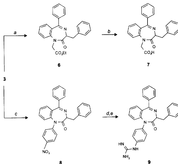
Scheme 2. Reagents and conditions: (a) (i) t -BuOK in THF (1M), THF, 0°C, N 2 , (ii) ethyl bromoacetate; (b) 1M KOH, EtOH, rt; (c) (i) 1-iodo-4-nitrobenzene, Cu powder, NaOAc, DMF, 150°C, 4h, (ii) 20h, rt; (d) SnCl 2 ·2H 2 O, EtOAc, 70°C, 16h; (e) (i) N,N' -di-Boc-thiourea, HgCl 2 , DMF, 20h, (ii) TFA, CH 2 Cl 2 .
