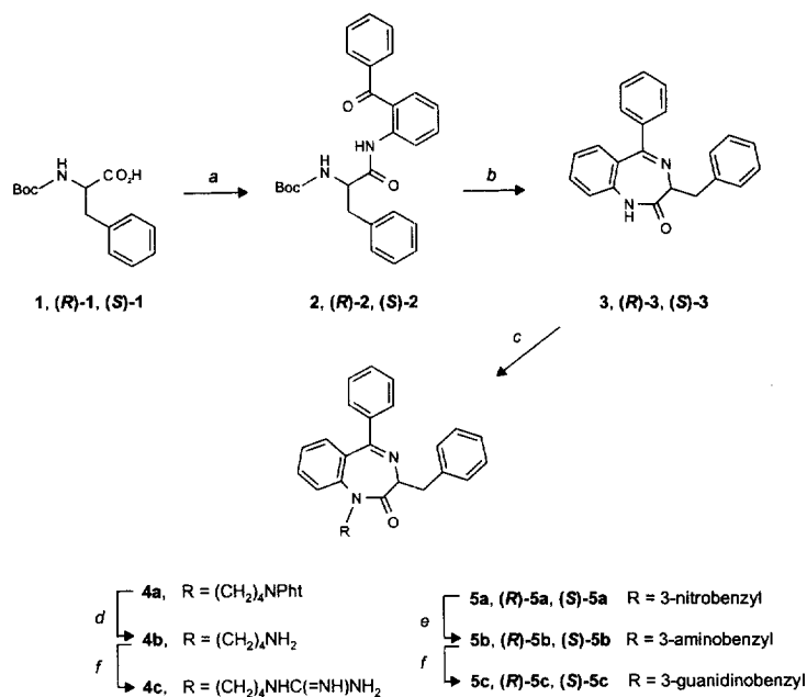
Scheme 1. Reagents and conditions: (a) (i) N -methylmorpholine, THF, -15°C, isobutyl chloroformate, (ii) 2-aminobenzophenone; (b) (i) HCl(g), EtOAc, 0°C, (ii) MeOH, 1M NaOH; (c) (i) t -BuOK in THF (1M), THF, 0°C, N 2 , (ii) N -(4-bromobutyl)phthalimide (for 4a) or 3-nitrobenzyl bromide (for 5a, (R)-5a, (S)-5a); (d) H 2 NNH 2 , EtOH; (e) SnCl 2 ·2H 2 O, EtOAc, 70°C, 16h; (f) (i) N,N' -di-Boc-thiourea, HgCl 2 , DMF, 18h, (ii) TFA, CH 2 Cl 2 .
